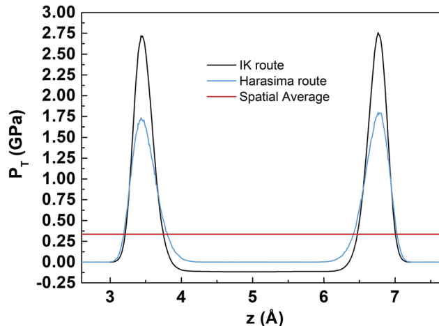
Fig. 1 Local tangential pressures using the IK and H definitions, and the spatially averaged tangential pressures (eqn (2)) for four different definitions of C_{ij} (the IK and H definitions, and two alternative contours), for LJ argon in a slit carbon pore of width H = 3\sigma at 87.3 K, 1 bar bulk pressure. 15
