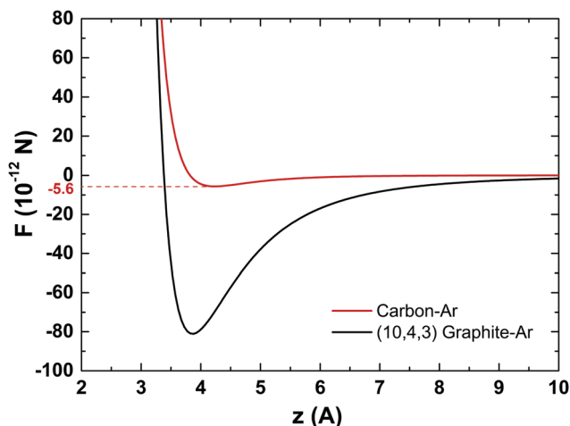
Fig. 3 Comparison of the isolated pair force between a carbon atom and an argon molecule with the total force on the Ar from all carbon atoms. The dashed line marks the minimum of the pair force.
