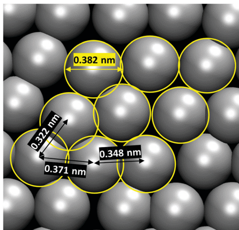
Fig. 2 An in-plane view of the contact layer next to the carbon wall for LJ argon in a carbon slit pore of width H = 3\sigma at 87.3 bar, 1 bar bulk pressure, showing separation distances between neighbouring molecules. The open circles show the nearest neighbor separation, 0.382 nm, when there is no compression, i.e. the intermolecular force is zero. Overlap of open circles implies strong repulsion between neighbouring pairs (see Fig. 4 of ref. 1 and 17).
