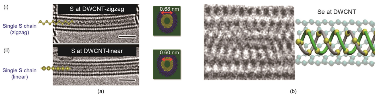
Fig. 4. (a) HRTEM images of sulfur (S) confined within carbon nanotubes: (i) Zigzag chain inside a DWCNT of 0.68 nm diameter; (ii) 1D linear sulfur chain inside a DWCNT of 0.60 nm diameter [56]. The scale bar is 1 nm. (b) Double-helix structure of selenium (Se) confined in a DWCNT with a diameter of about 1 nm [57]. (Adapted from Refs. [56,57])
